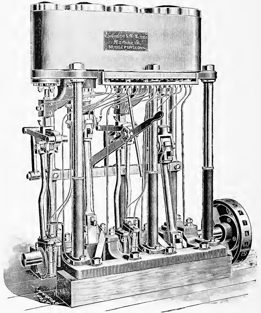
THE COULTER &amp; MCKENZIE COMPOUND ENGINE IN YACHT DREAM.
